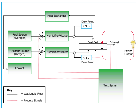
PEM fuel cell test station layout
