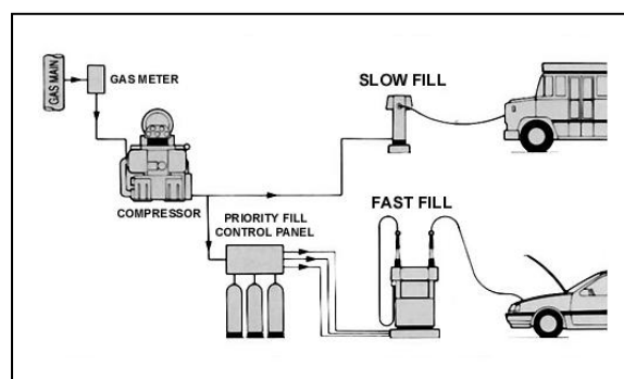
Typical CNG filling station layout
